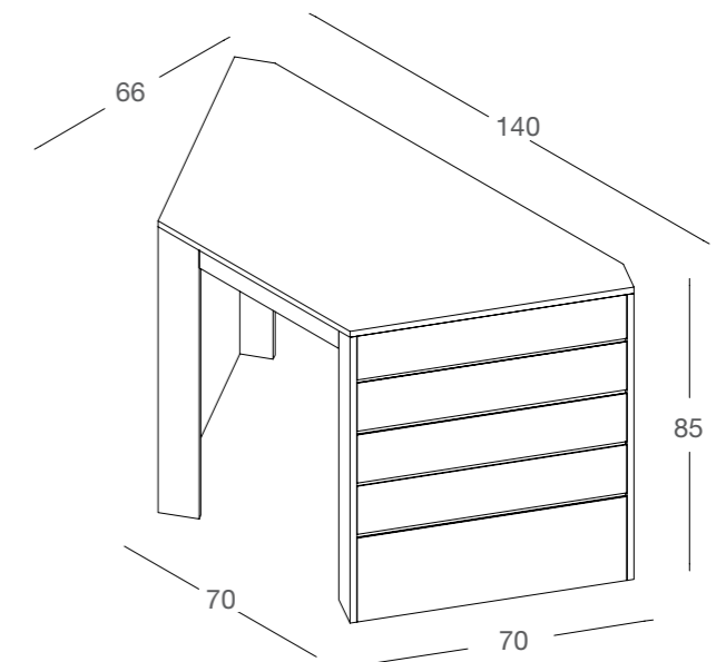
DGTT140 / L - N tavolo trapezio con fianchi dogati in nobilitato trapezoid-shaped table with slat-panel sides in faced panel L140 x P66 x H85 cm
