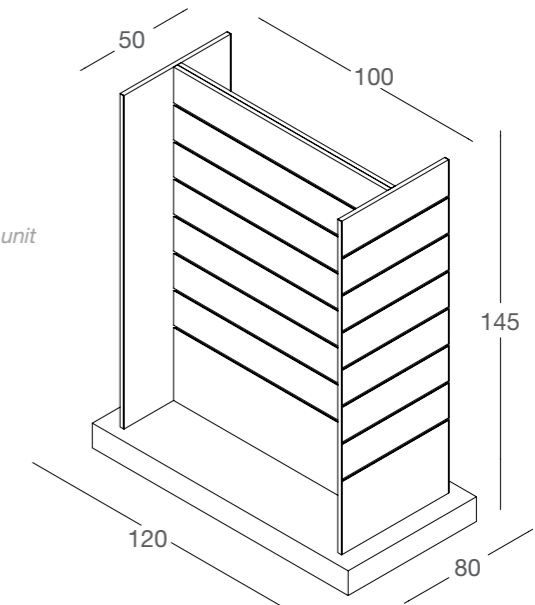
DGGH / L - N gondola acca in nobilitato H-shaped middle unit in faced panel L120 x P80 x H145 cm
