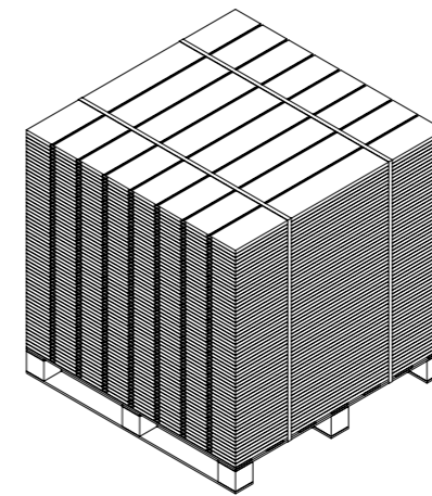
LARGE 60 pannelli panels 120 X 120 X H120 cm
